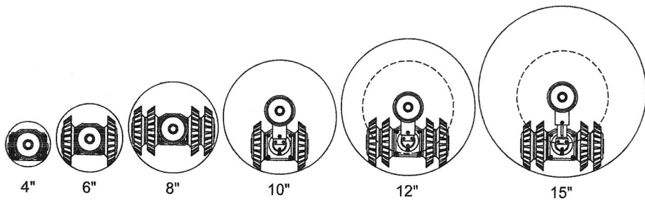
4" TRACTOR CONFIGURATIONS (4" - 15" PIPE)
